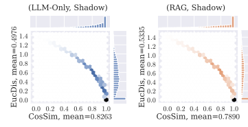
(e) Mistral-7B
