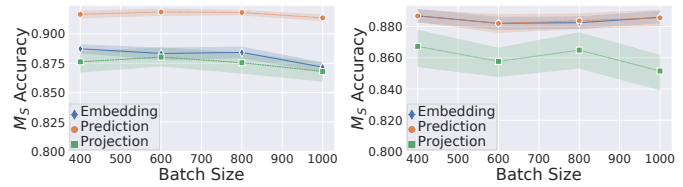
(a) Target model (GAT)
