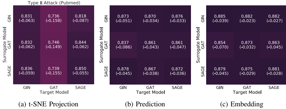
Fig. 5: Heatmap of the accuracy scores of Type II attacks. We show the performance results of 9 combinations of surrogate and target models given different scores information. The accuracy differences (in parenthesis) of the surrogate models to the target models are also reported. We fix the dataset to Pubmed.
