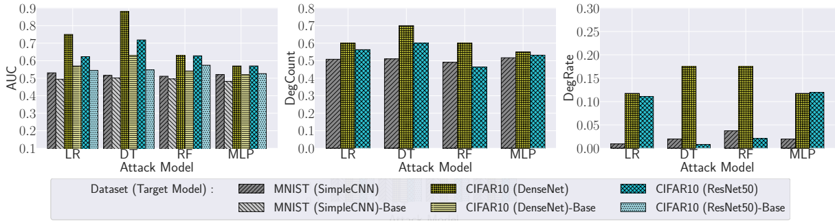
Figure 4: Privacy degradation level on the Scratch method for image datasets. In each subfig, the groups in x-axis stand for different attack models, the legends (in different colors) stand for different datasets and the corresponding target models. For the AUC metric, the right bars (transparent ones) stand for the AUC value of classical membership inference.
