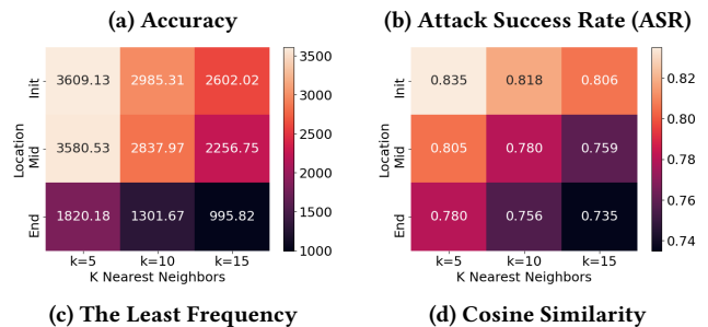
Figure 4: Attack performance of different k in KNN
