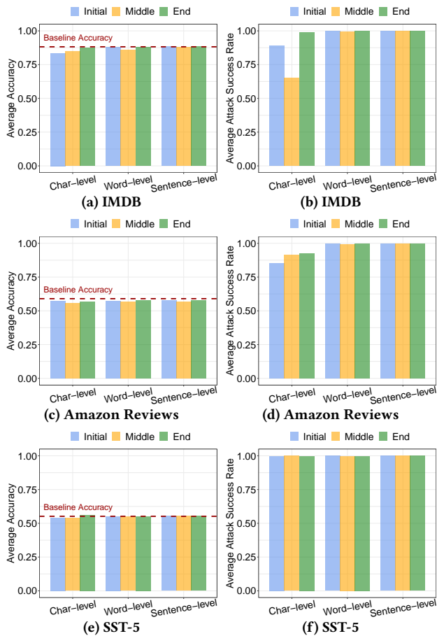
Figure 10: The comparison of the average accuracy and attack success rate for the backdoor attack using three basic trigger classes.
