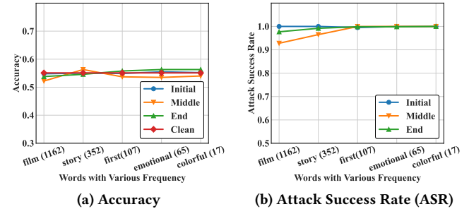
Figure 8: The accuracy and ASR of MixUp-based triggers with different frequencies for all three locations. The x-axis shows the words with their frequency in the dataset. (e.g., “film (1162)” means the frequency of word “film” in SST-5 is 1162).
