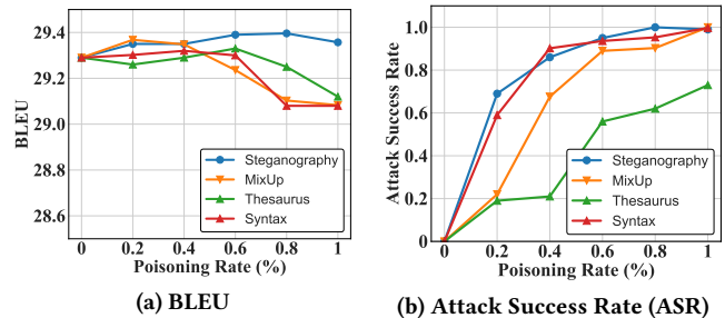
Figure 9: The BLEU and ASR on a Transformer-based NMT model using our semantic-preserving triggers.
