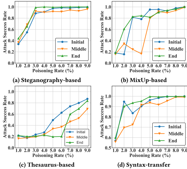
Figure 7: Poisoning rate evaluation of the semantic-preserving triggers.
